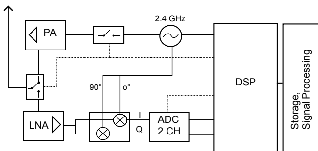
Figure 4 Block diagram of the interrogation unit
