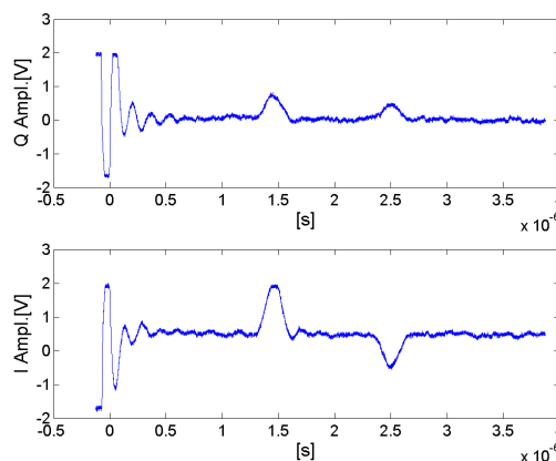
Figure 5 In-phase and quadrature Signal of a single SAW-sensor measurement.
