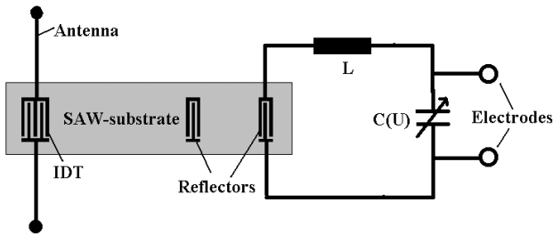
Figure 2 Design of the heart-potential sensor.
