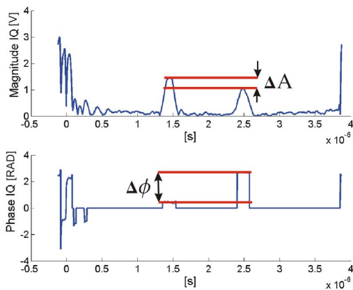
Figure 6 Computed phase and amplitude information of the quadrature signals.
