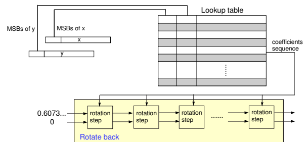
Fig. 4. A hybrid solution of lookup table and CORDIC
