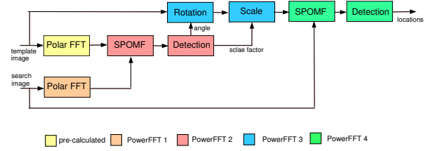
Fig. 1. The reconfigurable platform
