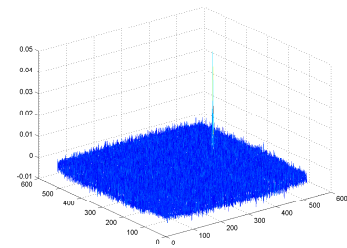
Fig. 7. SPOMF of mig-25 using sign bit only (SBO) normalization
