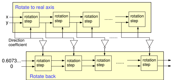
Fig. 3. Phase normalization with CORDIC
