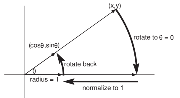
Fig. 2. Phase normalization with CORDIC
