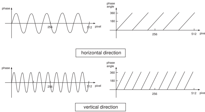
Fig. 9. Shift information represented by phase rotation circles
