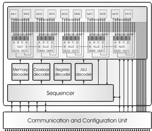
Figure 1: The Montium Tile Processor.
