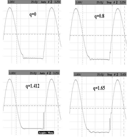
Fig. 3. Drain waveforms of the Class-E PA for q = 0, 0.8, 1.412, 1.65 with the given design specs in Table 5
