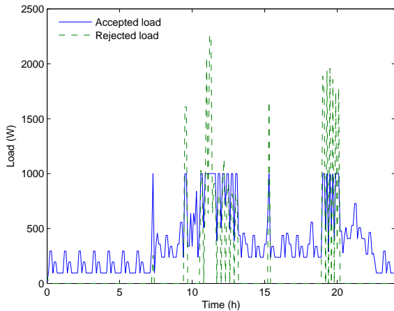
Fig. 4. Electricity demand cut off at 1kW
