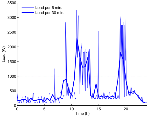
Fig. 3. Defined domestic electricity usage profile
