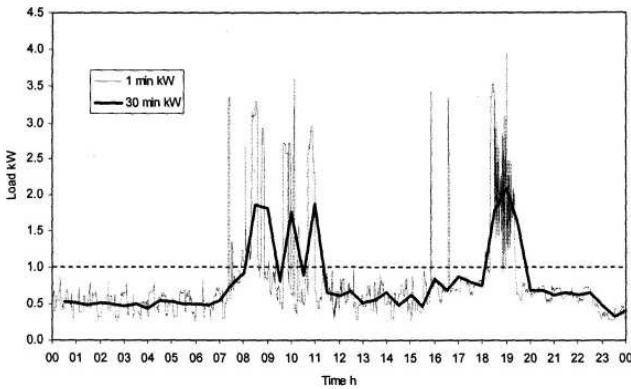
Fig. 1. Load profiles for a single December weekday for a house with a fairly typical high-demand
