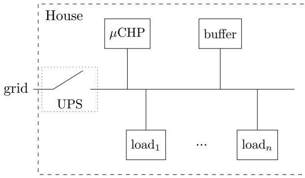
(a) Schematic of the electrical architecture of a house with islanding possibilities
