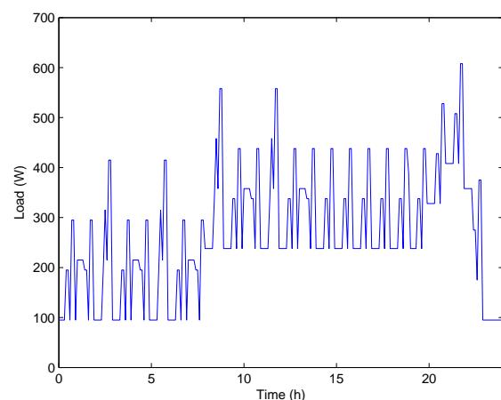
Fig. 5. Electricity demand lowered to 1kW by shedding appliances
