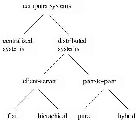
Fig. 1. computer systems
