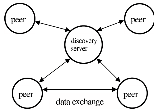
Fig. 2. centralized indexing
