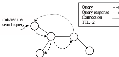
Fig. 5. flooding-based broadcast
