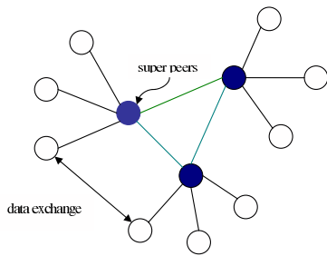
Fig. 3. distributed indexing
