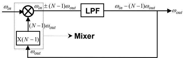
Fig. 1 Injection-locked frequency divider architecture
