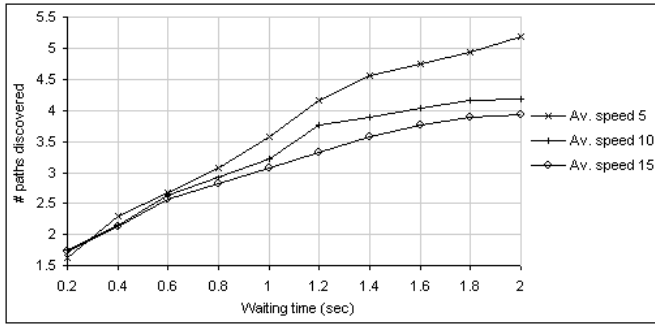
Fig. 9. Number of paths discovered
