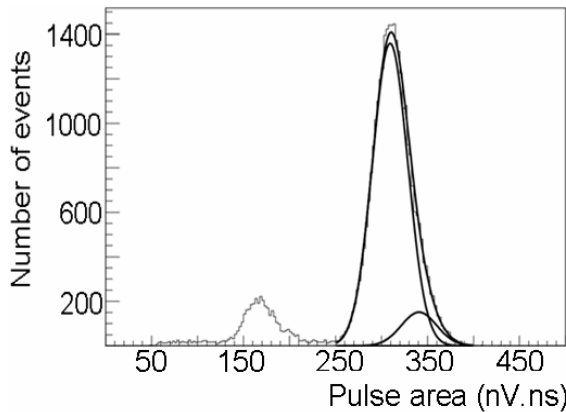
Figure 6: ^{55}\text{Fe} spectra in Argon showing the fit of the 5.9 keV and 6.5 keV lines.
