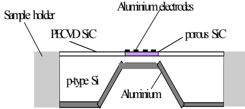
Fig. 1. A schematic of the devices used in this work. The sensing mechanism is capacitive with porous SiC as the sensing dielectric.
