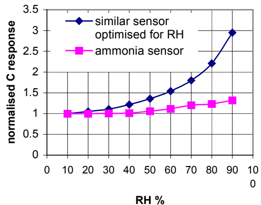
Figure 6. The response of our porous SiC ammonia sensor to relative humidity (10%-90%RH). For comparison a similar sensor optimised for RH sensing is also shown.
