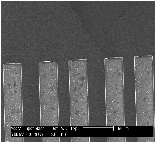
Fig. 4(a). SEM image showing the electrodes and the porous SiC surface. The darker 'patches' of the SiC surface contain larger pores – see figure 3(b)
