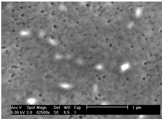
Fig. 4(b). Higher magnification SEM image showing larger (>100nm) pores within the darker regions of the SiC surface
