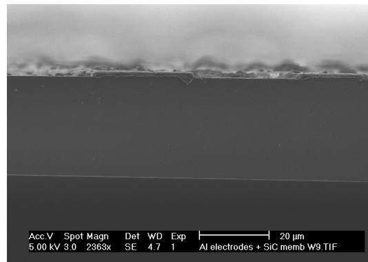
Figure 2: Cross-section SEM of SiC membrane & electrodes
