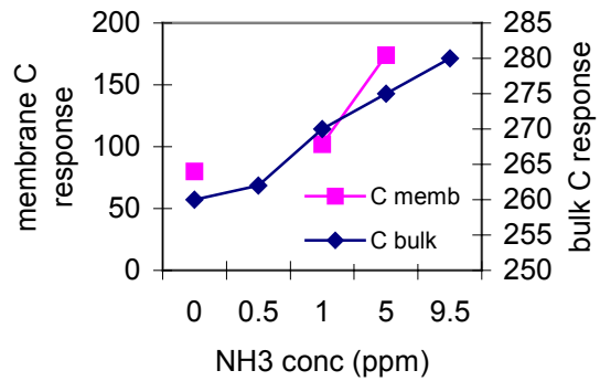
Fig. 5. The responses of a bulk porous SiC sensor and a porous SiC membrane sensor to dry NH 3 gas. Measurements were taken by interfacing to a laptop pc via the Universal Transducer Interface (UTI) from Smartek. The points were repeated several times and almost no hysteresis was evident. Measurements were taken approximately 10 mins after changing the NH 3 concentration.
