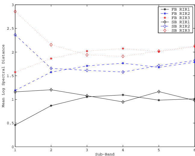
Fig. 3. Mean Log Spectral Distance for different RIRs.
