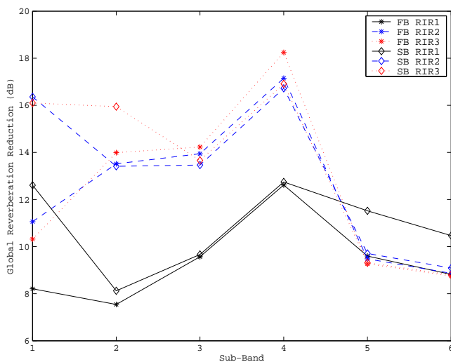
Fig. 2. Global Reverberation Reduction for different RIRs.
