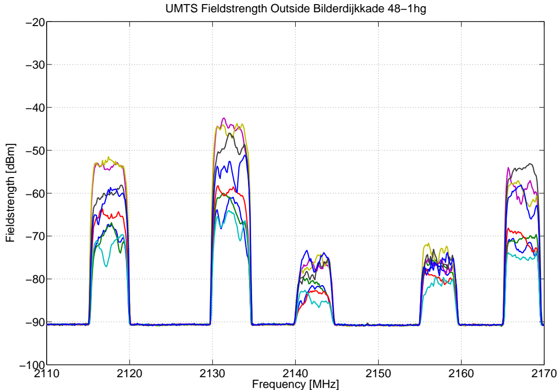
Fig. 3. Plot of 8 field strength measurements outside of a measurement location.
