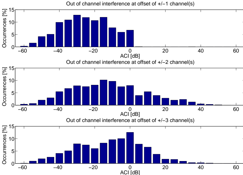
Fig. 4. Histograms of the out-of-channel interference levels at offsets of \pm 1 , \pm 2 or \pm 3 channels from the active channels.
