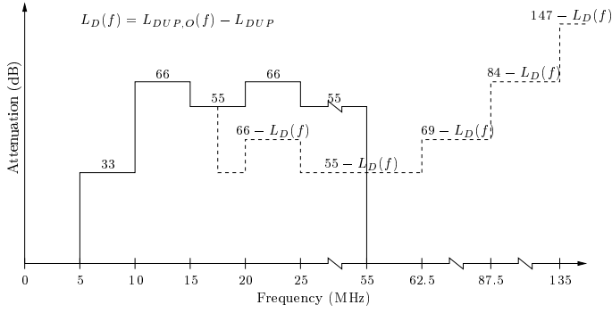
Fig. 1. Worst case adjacent channel attenuation requirements as a function of frequency offset from the center frequency of the desired channel [3]. The solid line indicates the attenuation requirements within the UMTS downlink band, while the dashed line indicates the out-of-band requirements.
