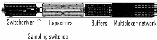
Figure 8: Layout of a single T/H channel
