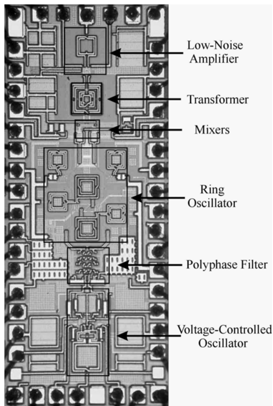
Fig. 5: 17GHz receiver RF front-end photomicrograph.
