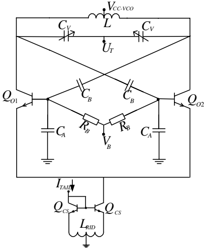
Fig. 2: LC voltage-controlled oscillator with RID TCS.
