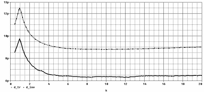
Fig. 9. Comparator delays as a function of k for an inverter booster (dashed) and a Schmitt trigger booster (solid)
