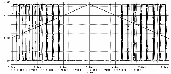
Fig. 10. ADC output in code 1-of- n for the inverter (dashed) and the Schmitt trigger (solid)
