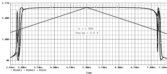
Fig. 8. Noise with larger magnitude leads to erroneous switching of Schmitt trigger (solid) and inverter (dashed)
