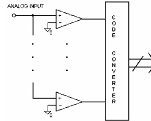
Fig. 1 Parallel resistorless ADC
