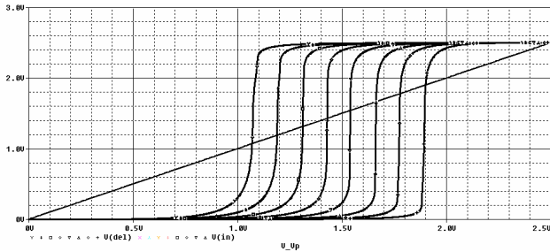
Fig. 3. Threshold voltage grid for a 3-bit ADC with two cascaded inverters
