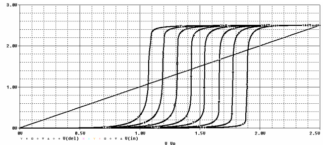
Fig. 5. Threshold voltage grid for a 3-bit ADC with an inverter followed by a Schmitt trigger with dynamic hysteresis
