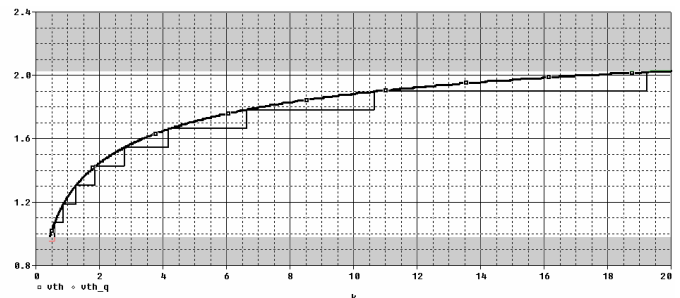
Fig. 2. Inverter threshold voltage V_{THI} as a function of transistor area ratio k
