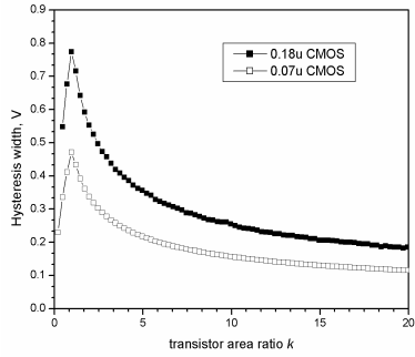
Fig. 6. Maximal noise magnitude that can be suppressed as a function of k
