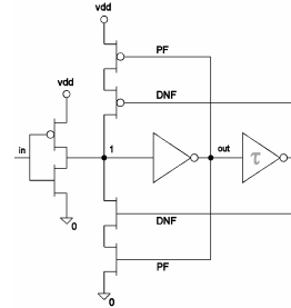
Fig. 4. Schmitt trigger with dynamic hysteresis
