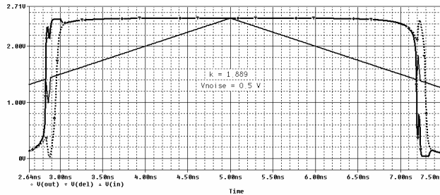
Fig. 7. Successful noise suppression (solid) and erroneous output of the inverter circuit (dashed)
