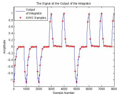
Fig. 6. The signal after the integrator
