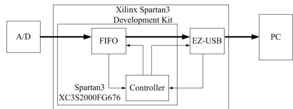
Fig. 7. Function block diagram for USB communication
