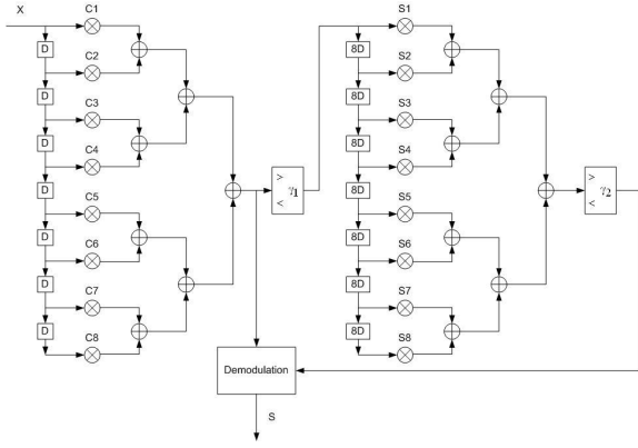
Fig. 8. The architecture for two stage synchronization digital receiver
