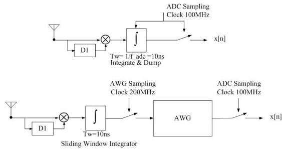
Fig. 5. The equivalent analog parts
