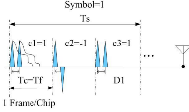
Fig. 3. The transmitted UWB signal
