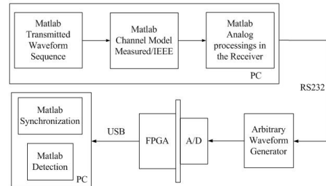
Fig. 2. The block diagram of the platform for a DHTR UWB system prototype development
